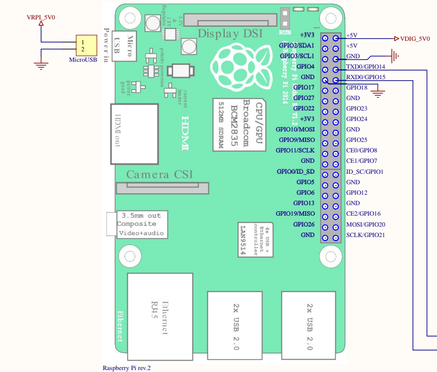
Raspberry Pi rev.2
